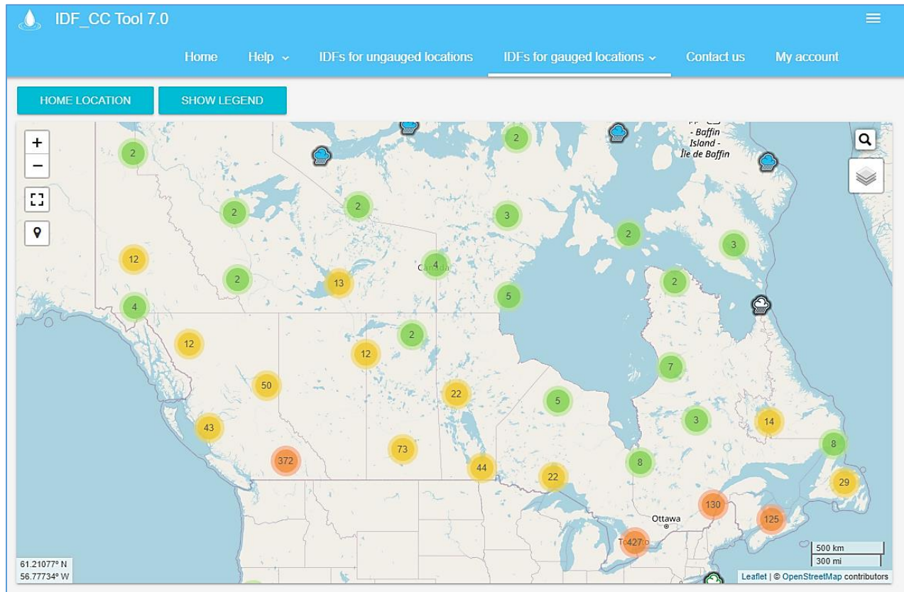
Figure 2. Screenshot of the IDF_CC tool version 7.0 user interface
